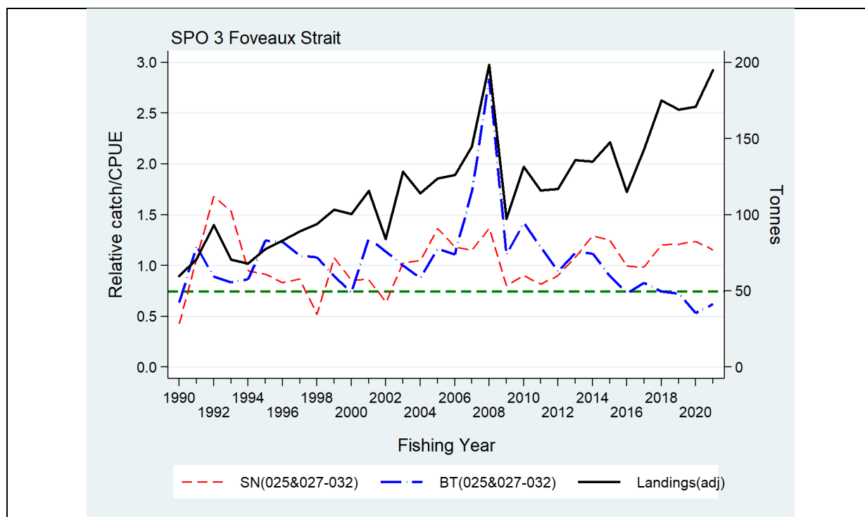
Relative fishing pressure for Foveaux Strait SPO 3 based on the ratio of QMR/MHR (adj) landings (sum of areas 025&027–032) relative to the SN(025&027–032) and BT(025&027–032) CPUE series which have been normalised so that the geometric mean=1.0. The indicated threshold (green dashed line) is geometric average fishing pressure from 2002 to 2012 for the SN(025&027–032) series divided by 1.333.
